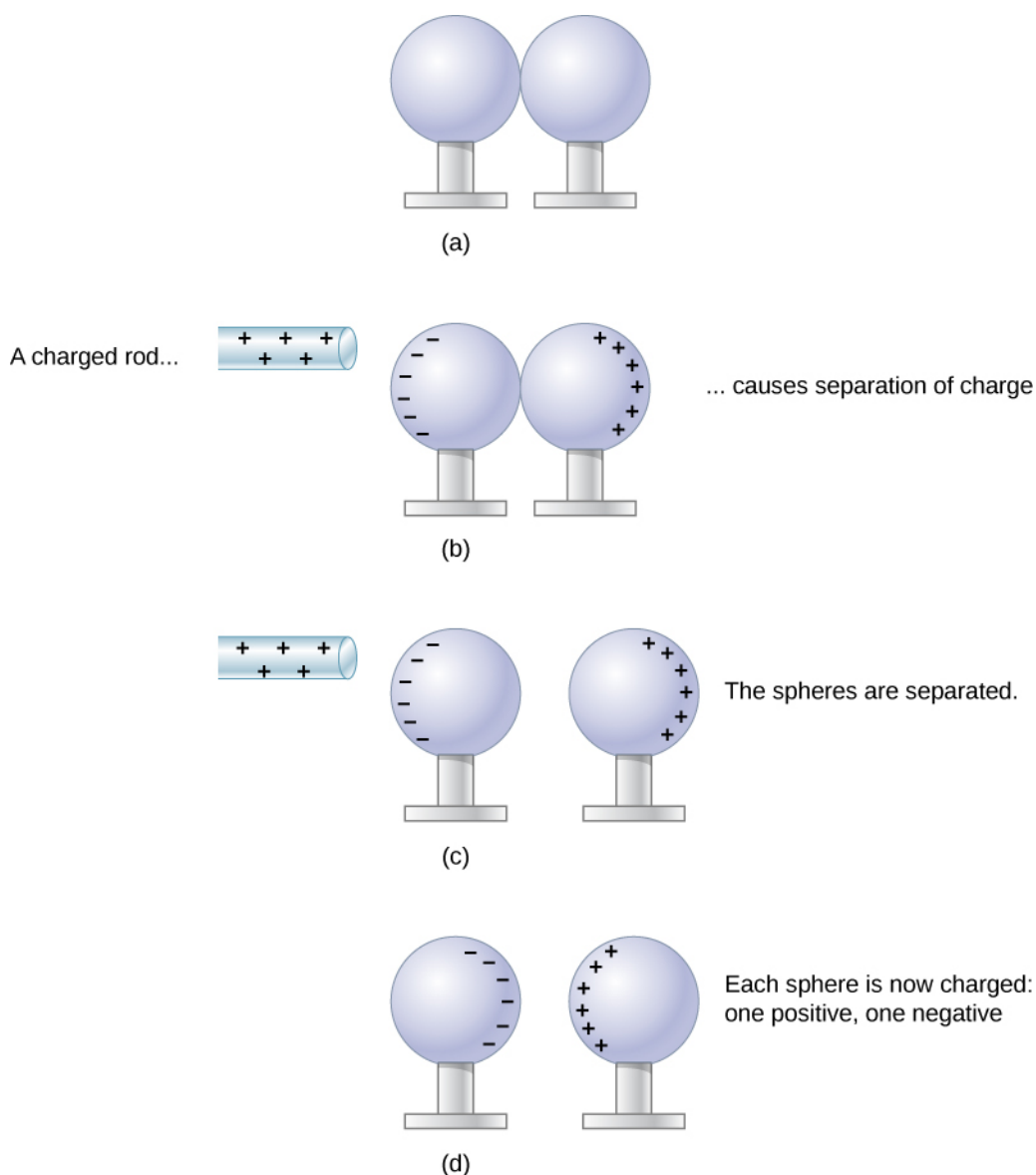
Figure 5.12 Charging by induction. (a) Two uncharged or neutral metal spheres are in contact with each other but insulated from the rest of the world. (b) A positively charged glass rod is brought near the sphere on the left, attracting negative charge and leaving the other sphere positively charged. (c) The spheres are separated before the rod is removed, thus separating negative and positive charges. (d) The spheres retain net charges after the inducing rod is removed—without ever having been touched by a charged object.
