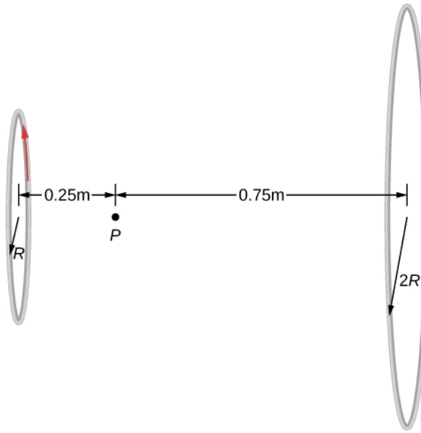
Figure 12.13 Two loops of different radii have the same current but flowing in opposite directions. The magnetic field at point P is measured to be zero.
